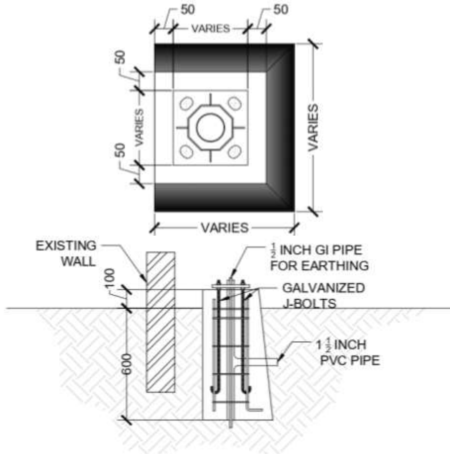
FOOTING SECTION SCALE 1:20
